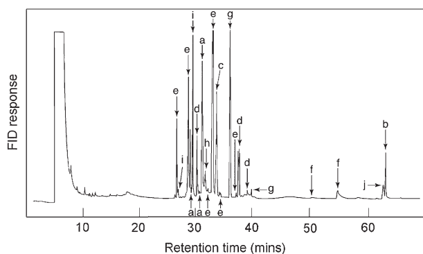
Fig. 3. Chromatogram of sugar derivatives from extract of mixed sugar standards (multiple peaks of the same sugar, anomeric forms). a, Fructose; b, sucrose; c, galactose; d, mannose; e, gulose; f, raffinose; g, glucose; h, allose; i, altrose; j, lactose; FID, flame ionization detector.
